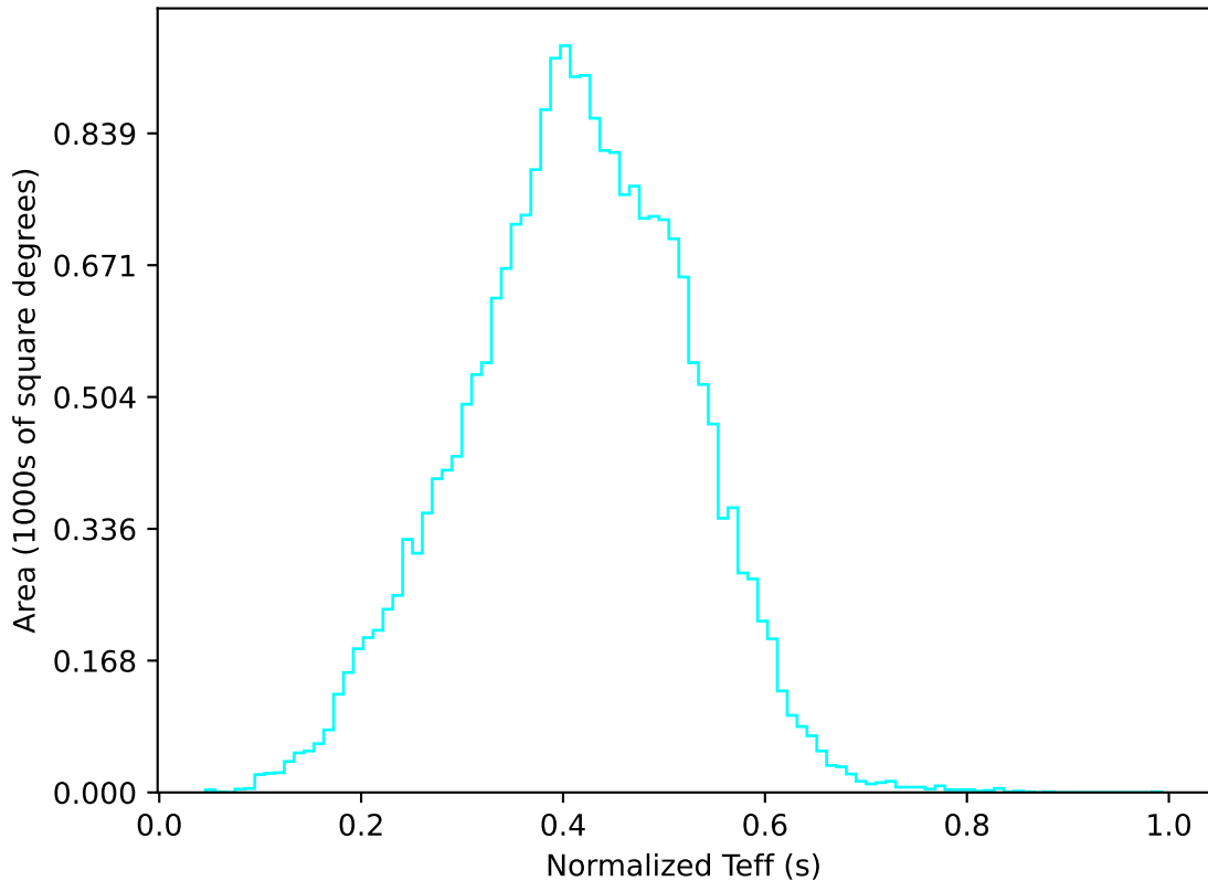
too_elab_r32_d3_griz_v3.4_10yrs All sky u band: Normalized Teff
