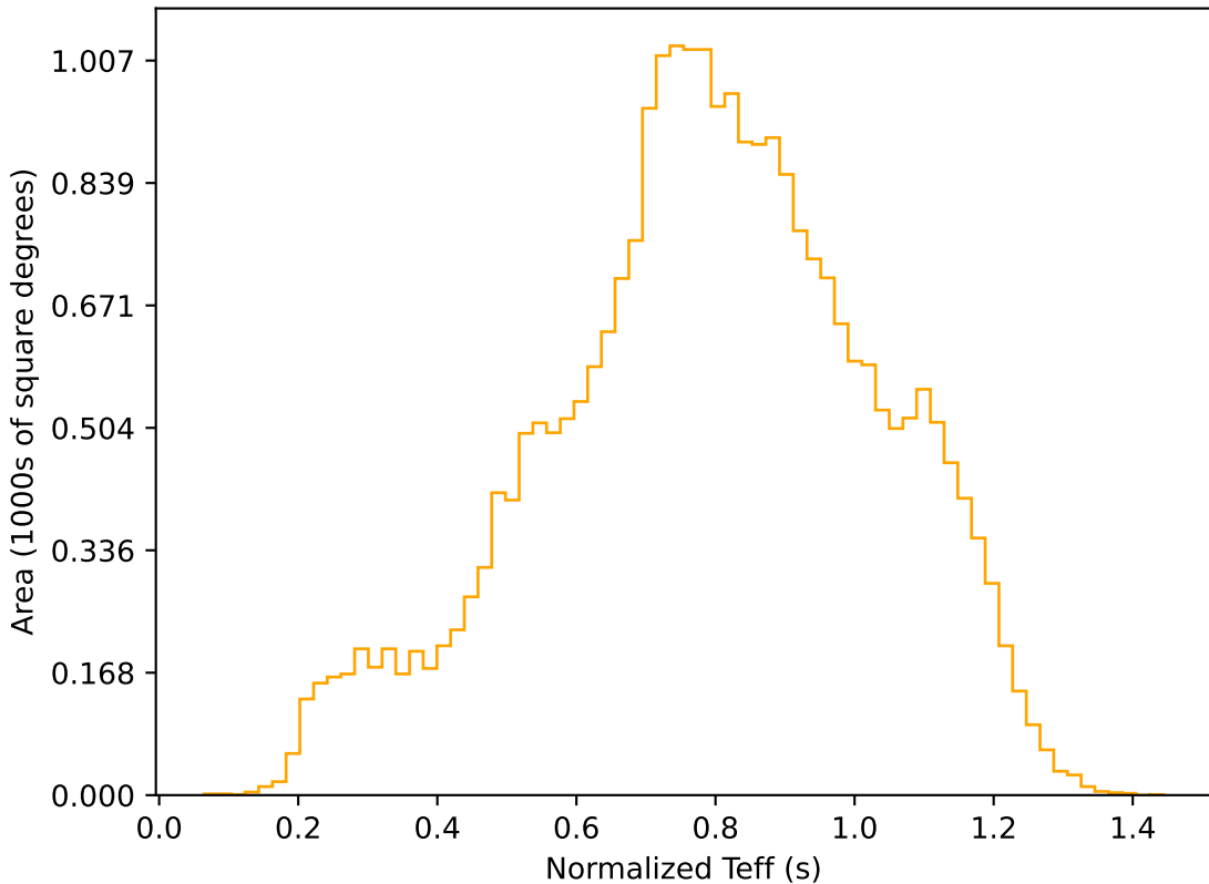
too_elab_r32_d3_griz_v3.4_10yrs All sky r band: Normalized Teff
