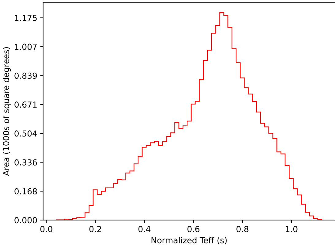
too_elab_r32_d3_griz_v3.4_10yrs All sky i band: Normalized Teff
