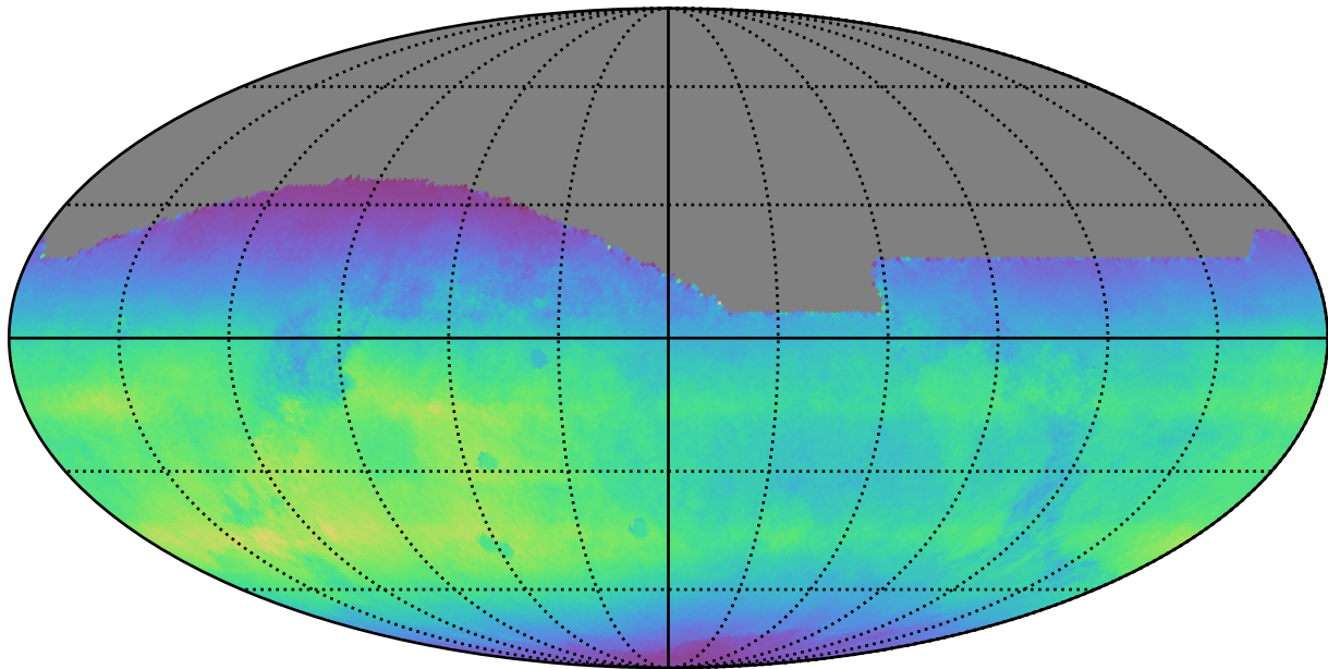
too_elab_r32_d3_griz_v3.4_10yrs All sky all bands: Normalized Teff
