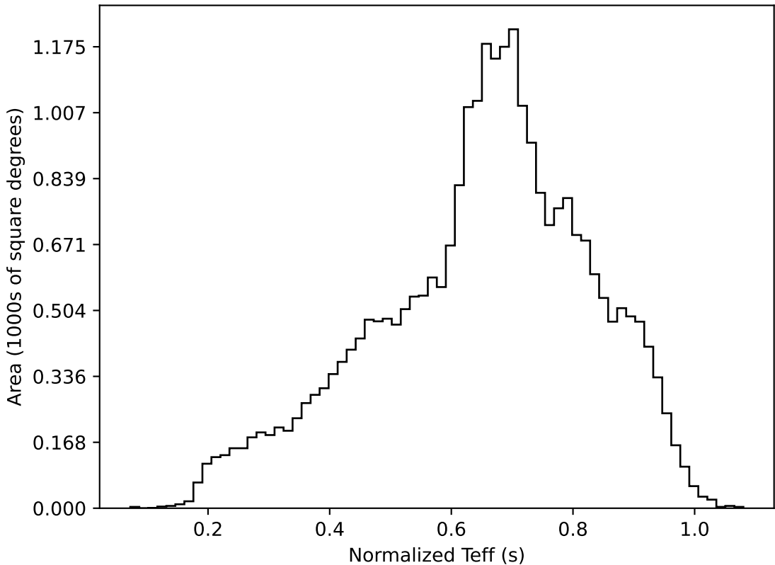
too_elab_r32_d3_griz_v3.4_10yrs All sky all bands: Normalized Teff
