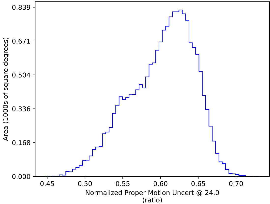
too_elab_r32_d3_griz_v3.4_10yrs WFD: Normalized Proper Motion Uncert @ 24.0
