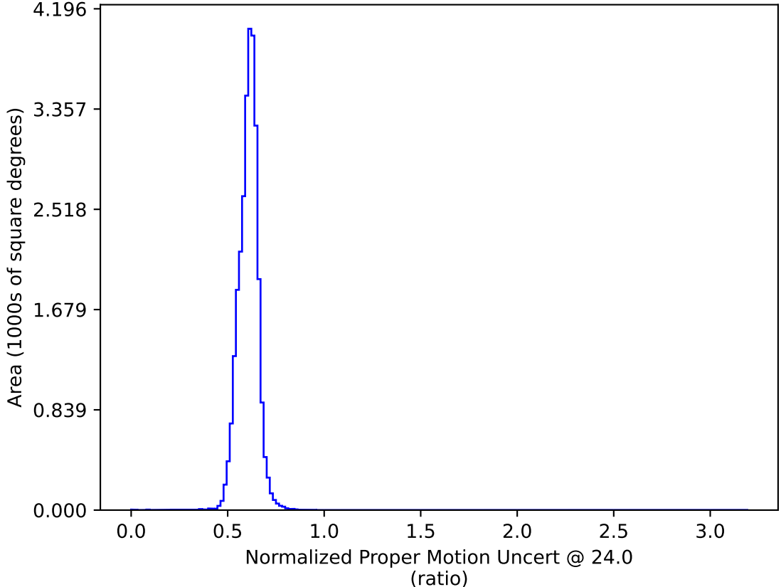
too_elab_r32_d3_griz_v3.4_10yrs All sky: Normalized Proper Motion Uncert @ 24.0
