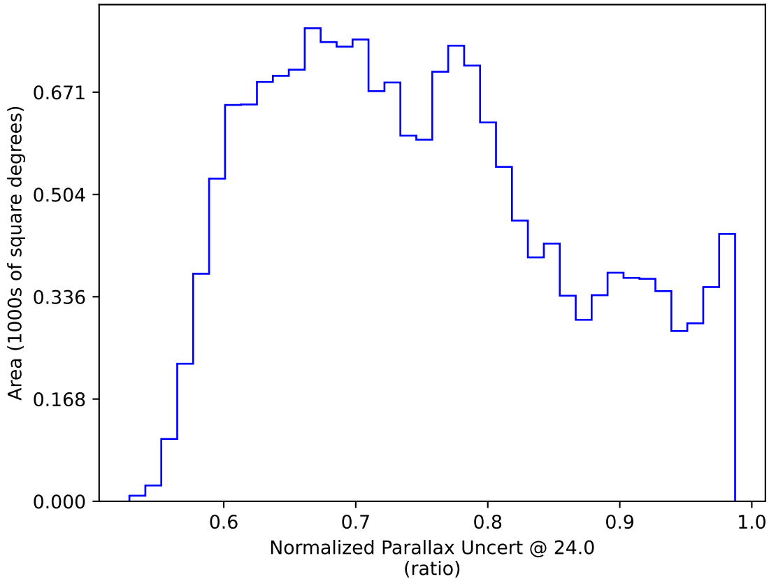
too_elab_r32_d3_griz_v3.4_10yrs WFD: Normalized Parallax Uncert @ 24.0
