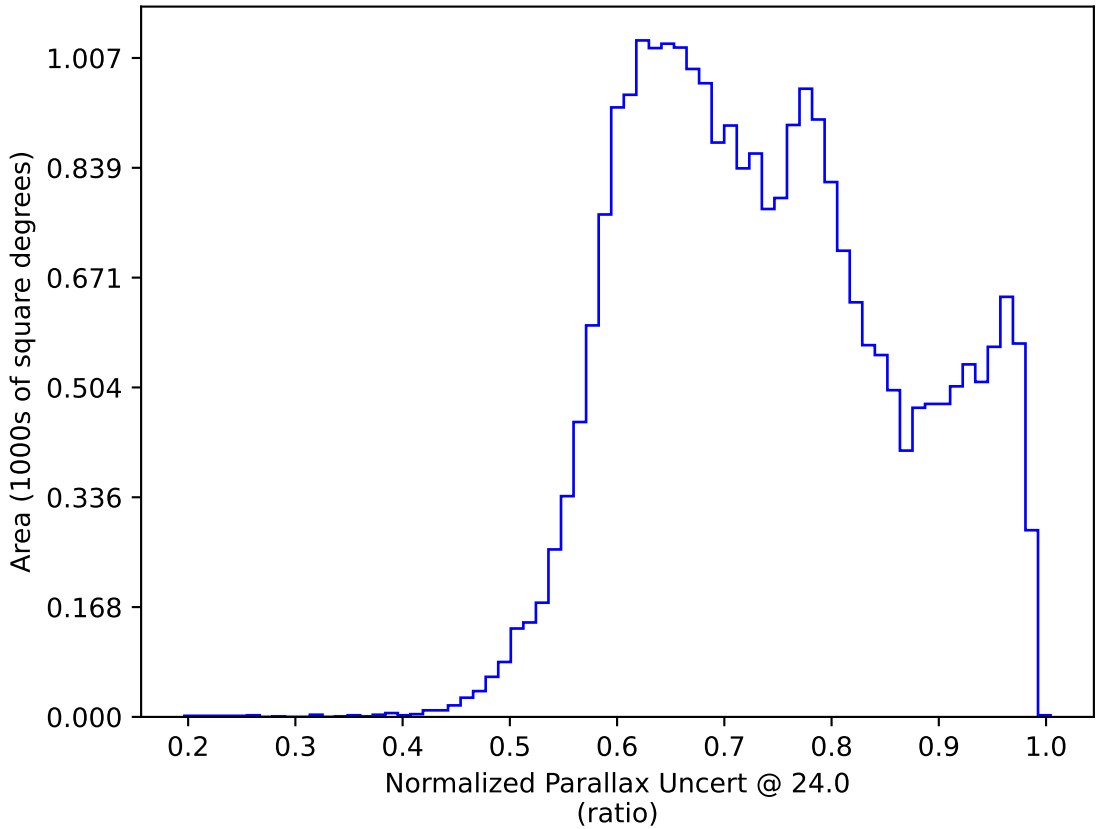
too_elab_r32_d3_griz_v3.4_10yrs All sky: Normalized Parallax Uncert @ 24.0
