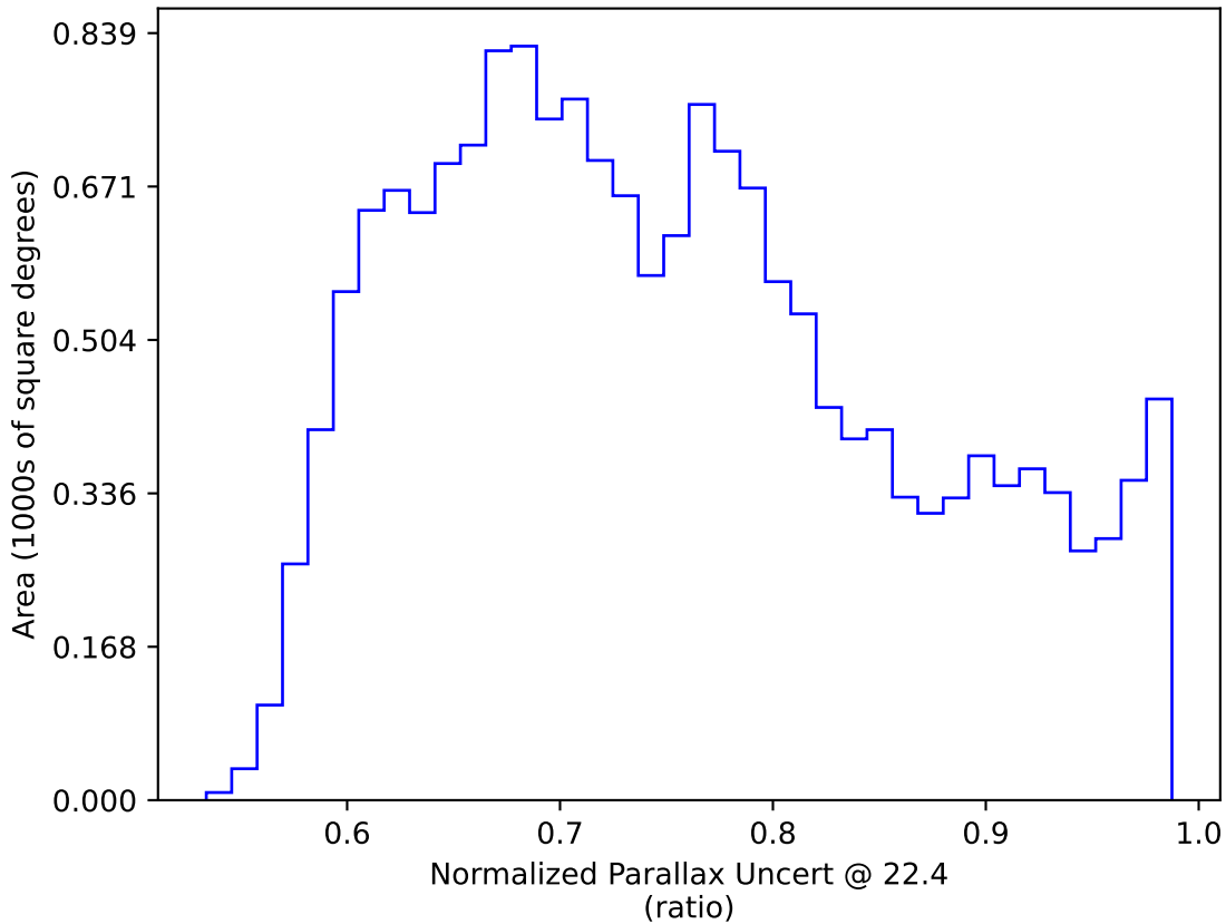
too_elab_r32_d3_griz_v3.4_10yrs WFD: Normalized Parallax Uncert @ 22.4
