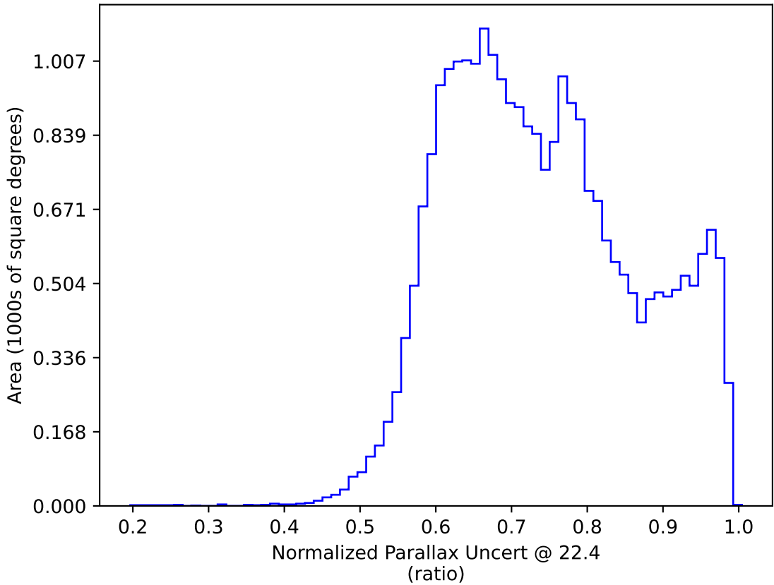
too_elab_r32_d3_griz_v3.4_10yrs All sky: Normalized Parallax Uncert @ 22.4
