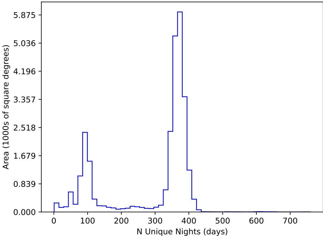
too_elab_r32_d3_griz_v3.4_10yrs All sky all bands: N Unique Nights
