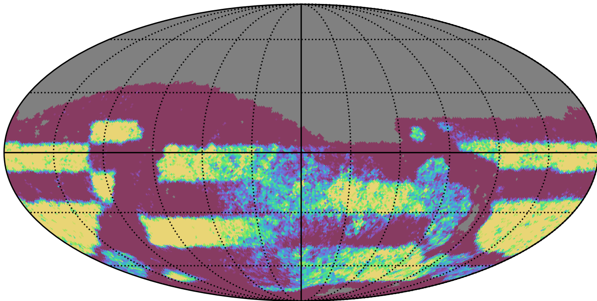
too_elab_r32_d3_griz_v3.4_10yrs Yr 3-4 r band: NVisits
