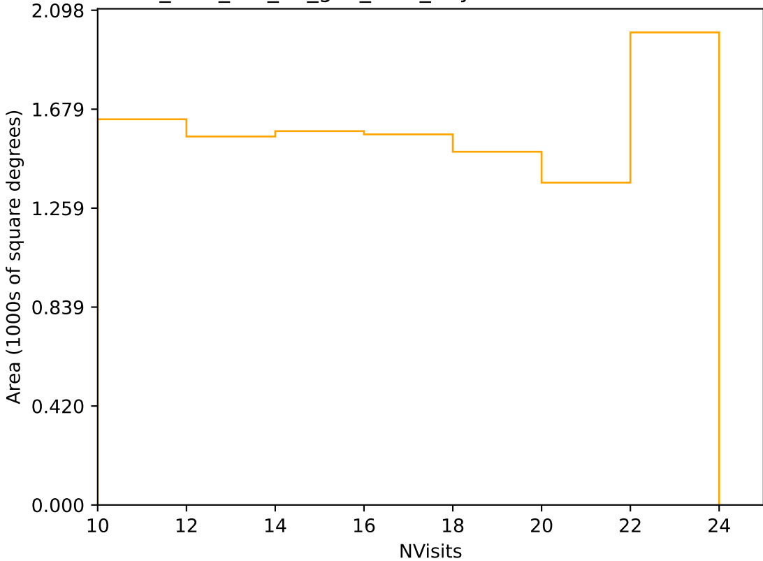
too_elab_r32_d3_griz_v3.4_10yrs Yr 3-4 r band: NVisits
