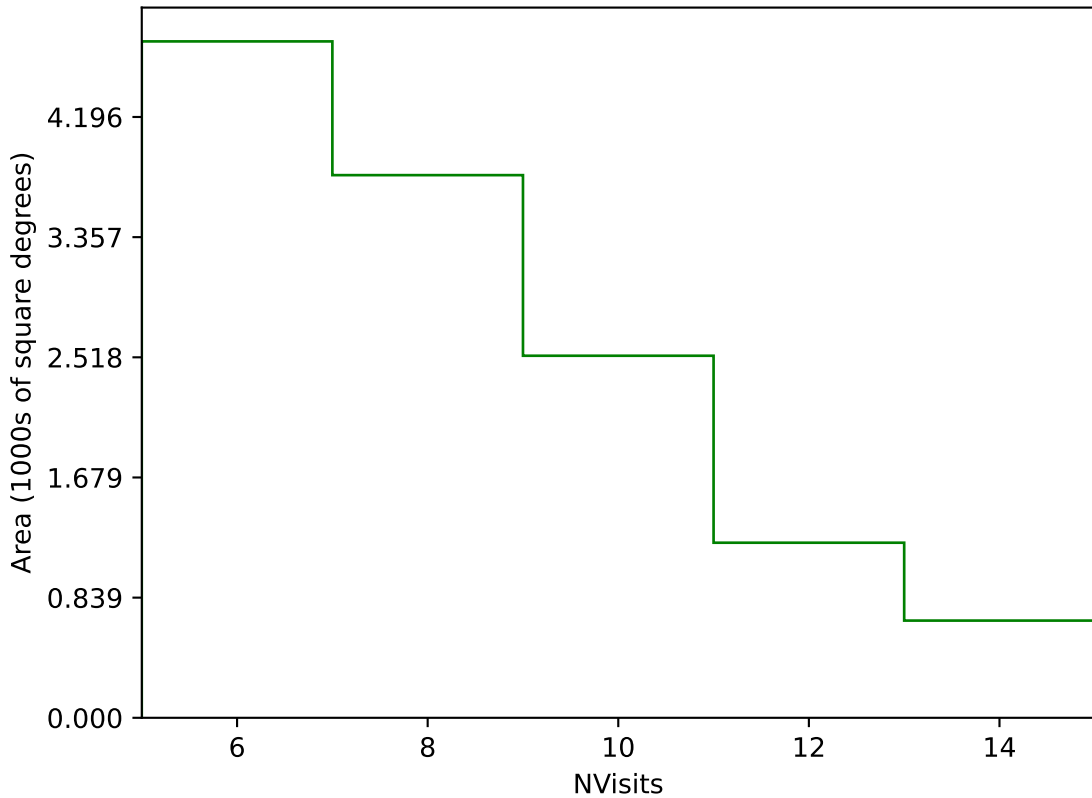
too_elab_r32_d3_griz_v3.4_10yrs Yr 3-4 g band: NVisits
