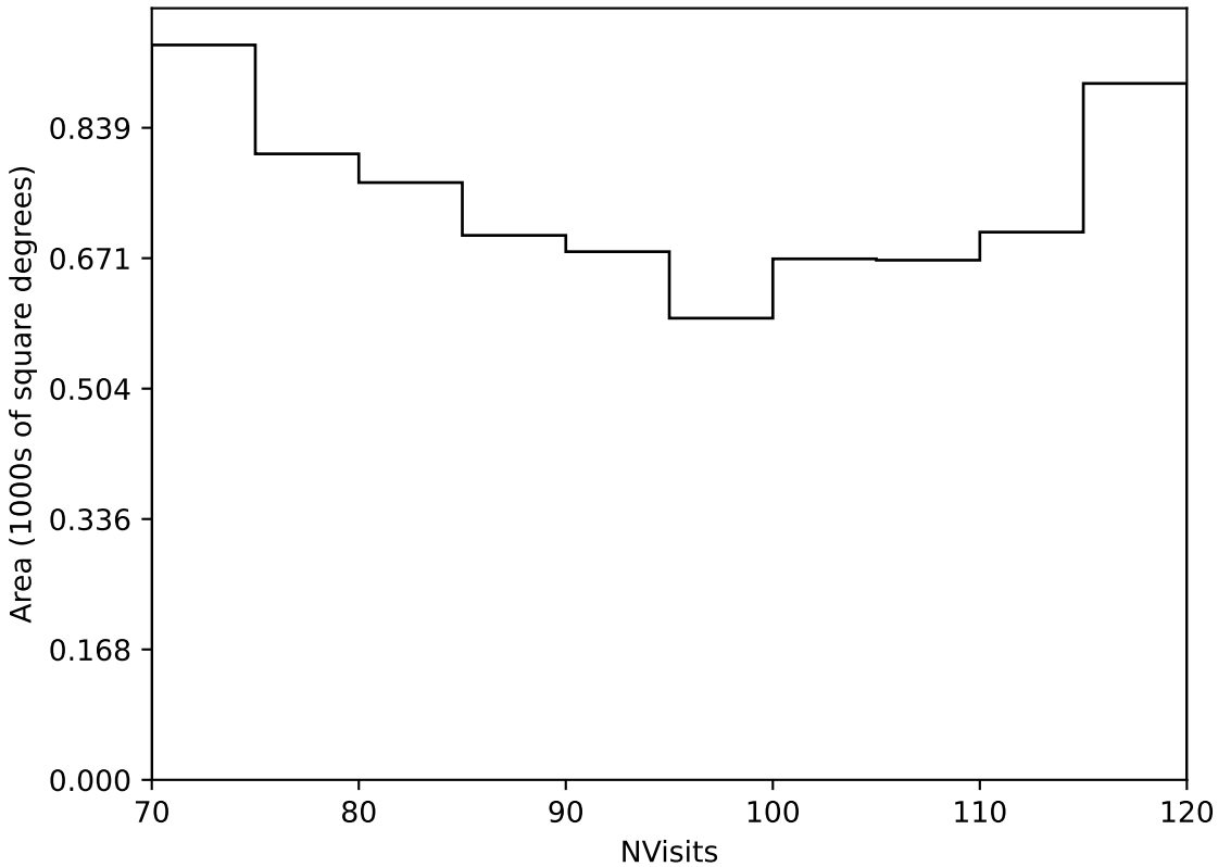
too_elab_r32_d3_griz_v3.4_10yrs Yr 3-4 all bands: NVisits
