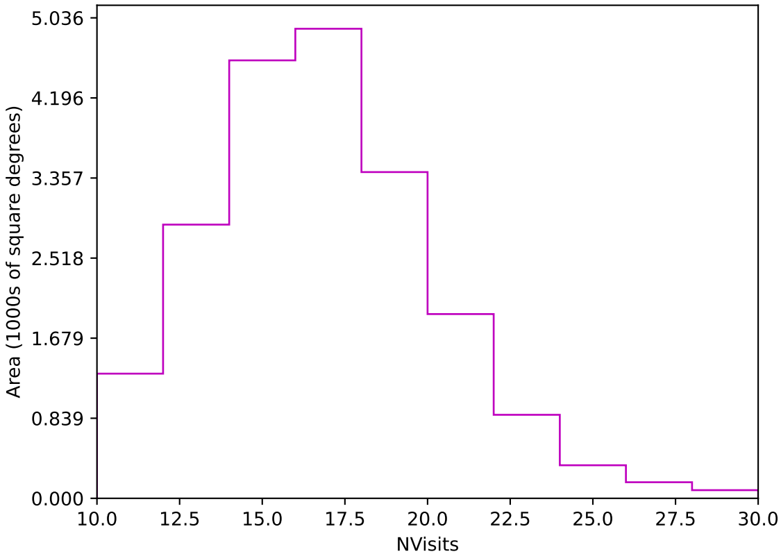
too_elab_r32_d3_griz_v3.4_10yrs Yr 1 z band: NVisits
