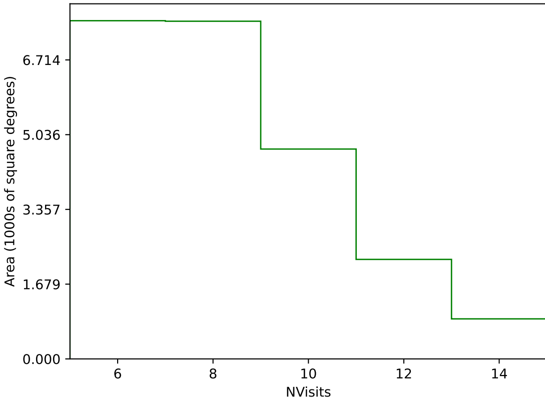
too_elab_r32_d3_griz_v3.4_10yrs Yr 1 g band: NVisits
