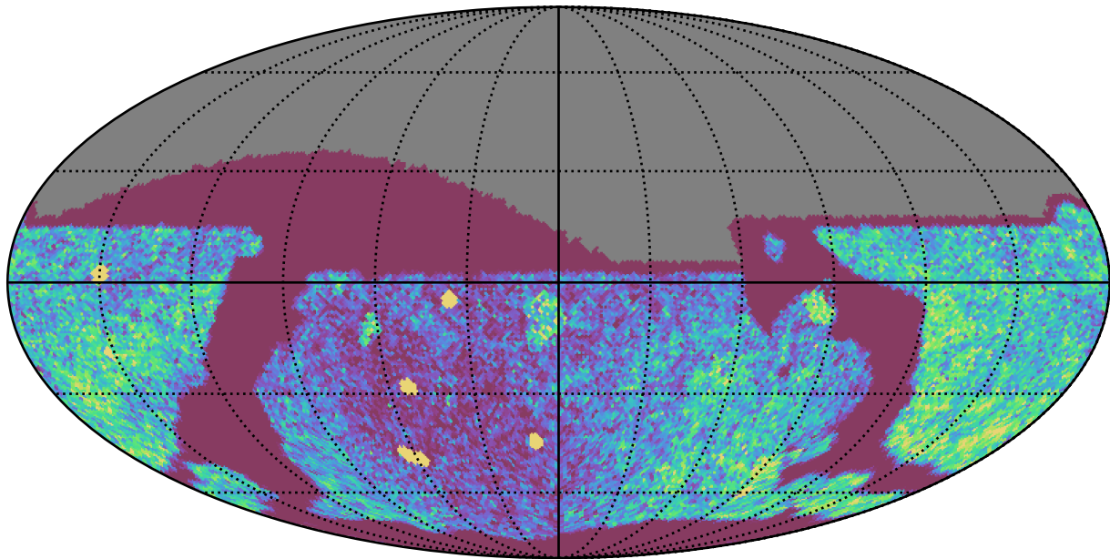
too_elab_r32_d3_griz_v3.4_10yrs Yr 1 all bands: NVisits
