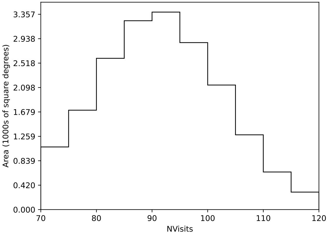
too_elab_r32_d3_griz_v3.4_10yrs Yr 1 all bands: NVisits
