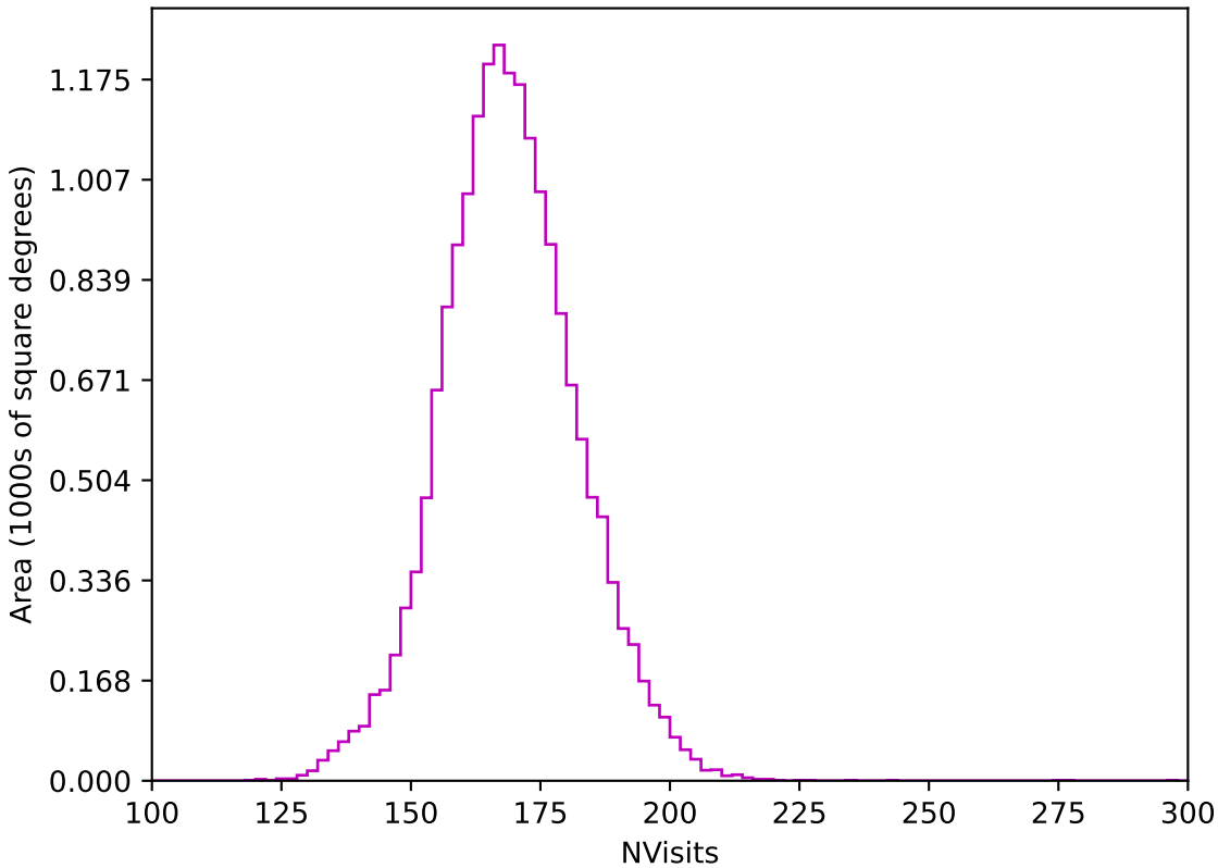
too_elab_r32_d3_griz_v3.4_10yrs WFD z band: NVisits
