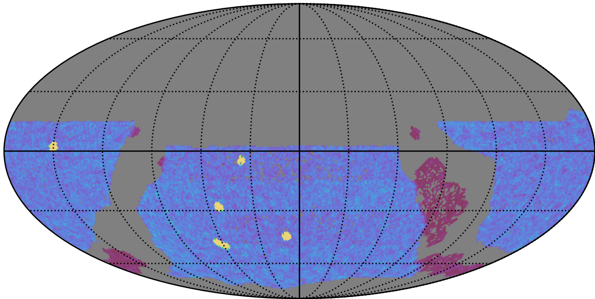
too_elab_r32_d3_griz_v3.4_10yrs WFD y band: NVisits
