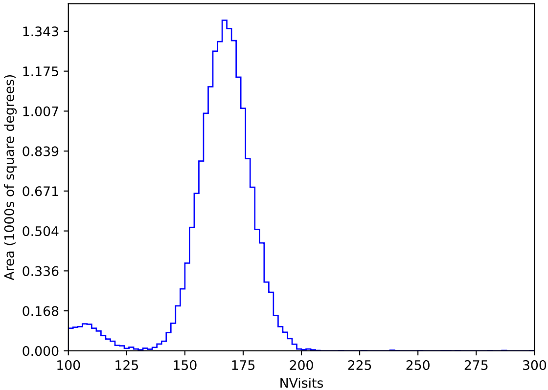
too_elab_r32_d3_griz_v3.4_10yrs WFD y band: NVisits
