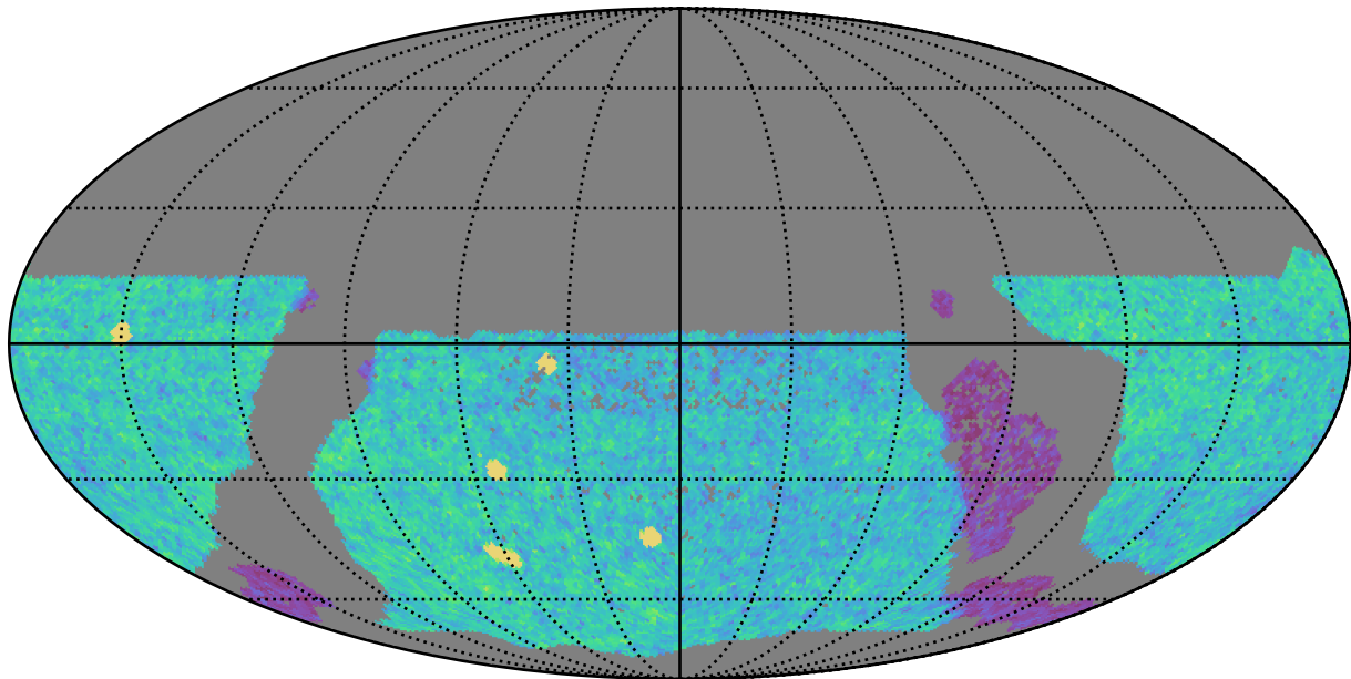
too_elab_r32_d3_griz_v3.4_10yrs WFD u band: NVisits
