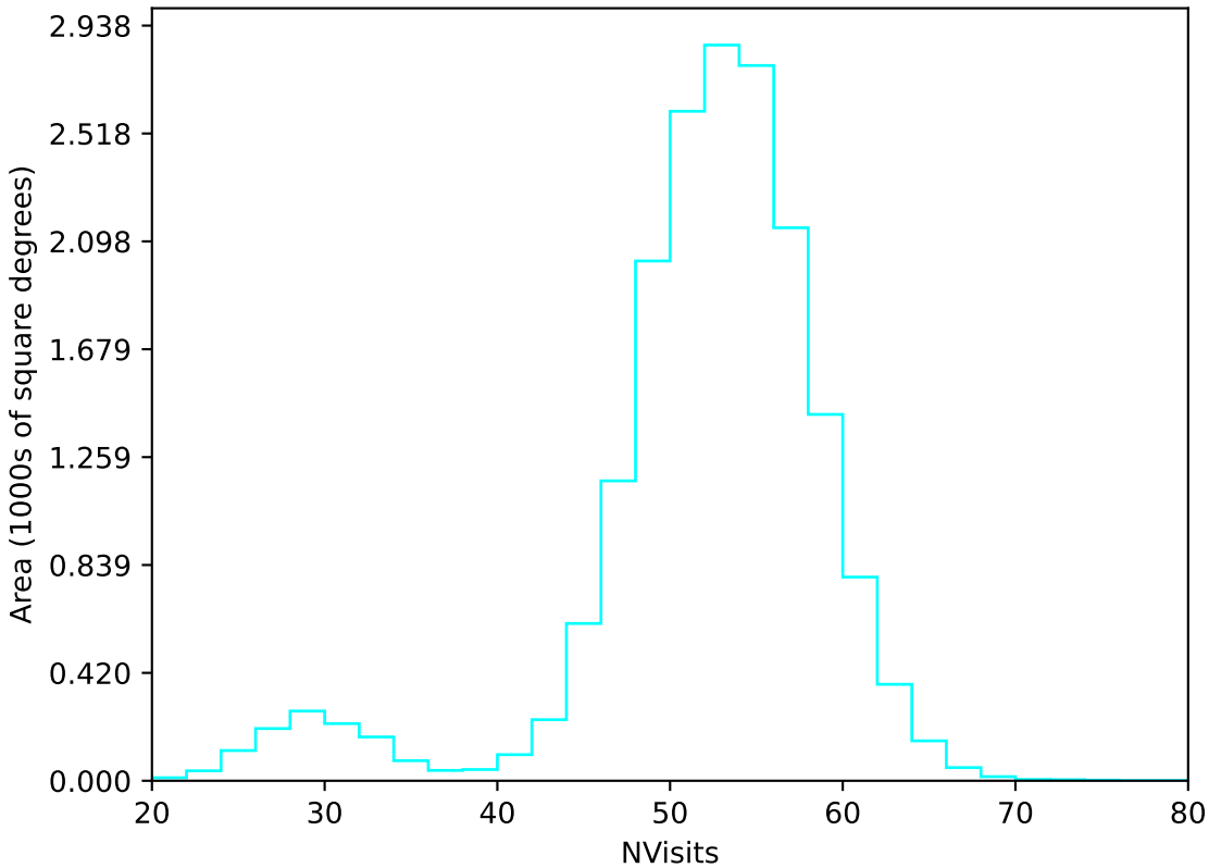
too_elab_r32_d3_griz_v3.4_10yrs WFD u band: NVisits
