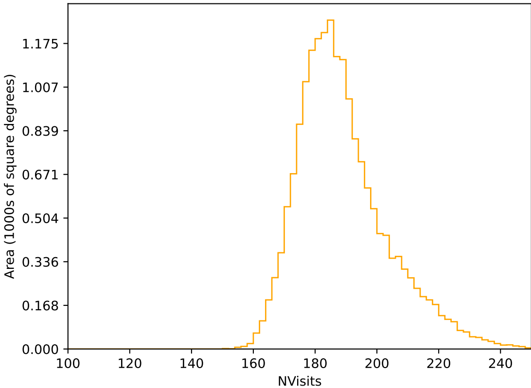
too_elab_r32_d3_griz_v3.4_10yrs WFD r band: NVisits
