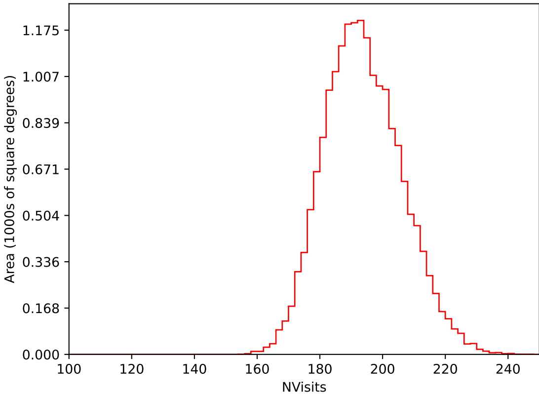
too_elab_r32_d3_griz_v3.4_10yrs WFD i band: NVisits
