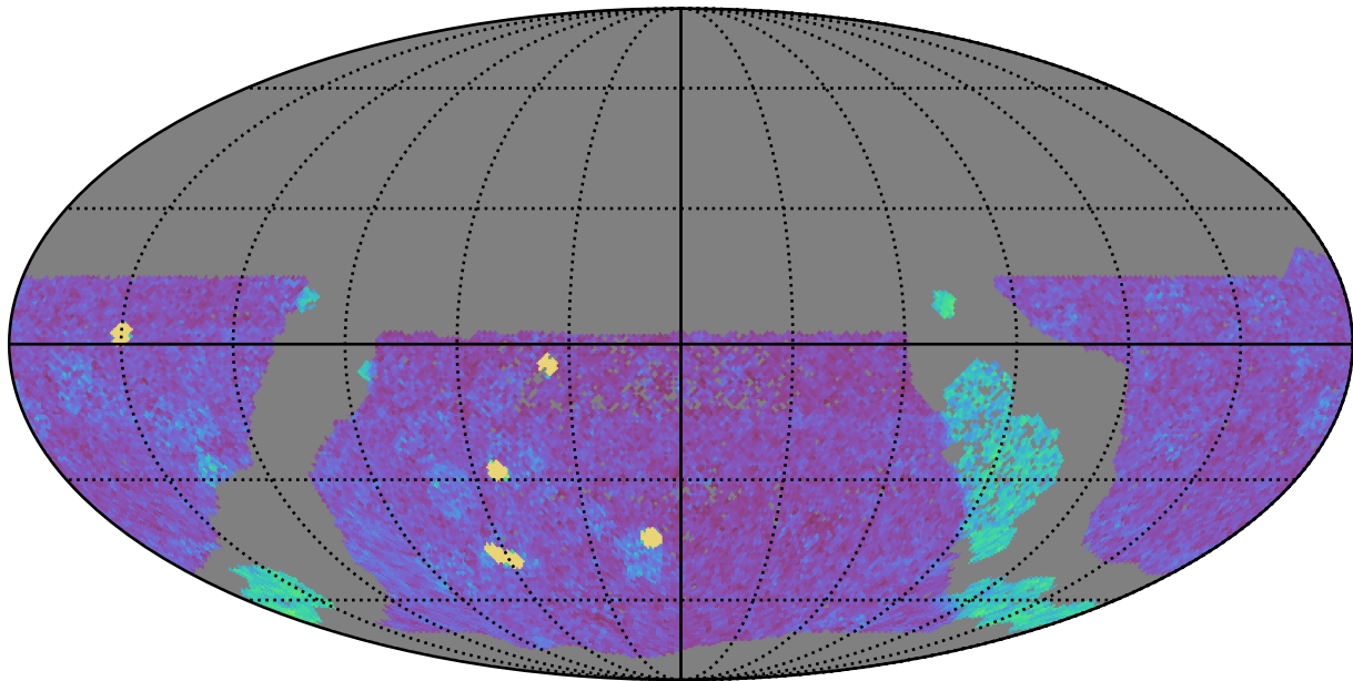
too_elab_r32_d3_griz_v3.4_10yrs WFD g band: NVisits
