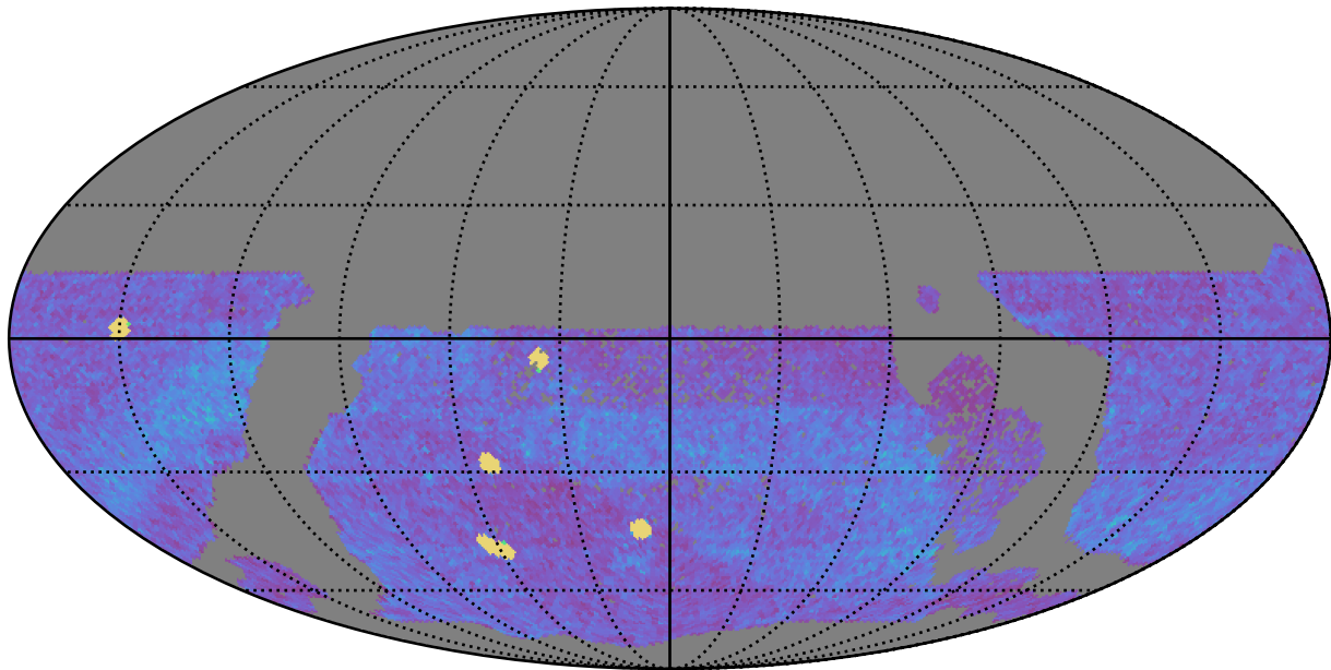
too_elab_r32_d3_griz_v3.4_10yrs WFD all bands: NVisits
