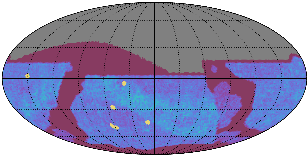
too_elab_r32_d3_griz_v3.4_10yrs All sky z band: NVisits
