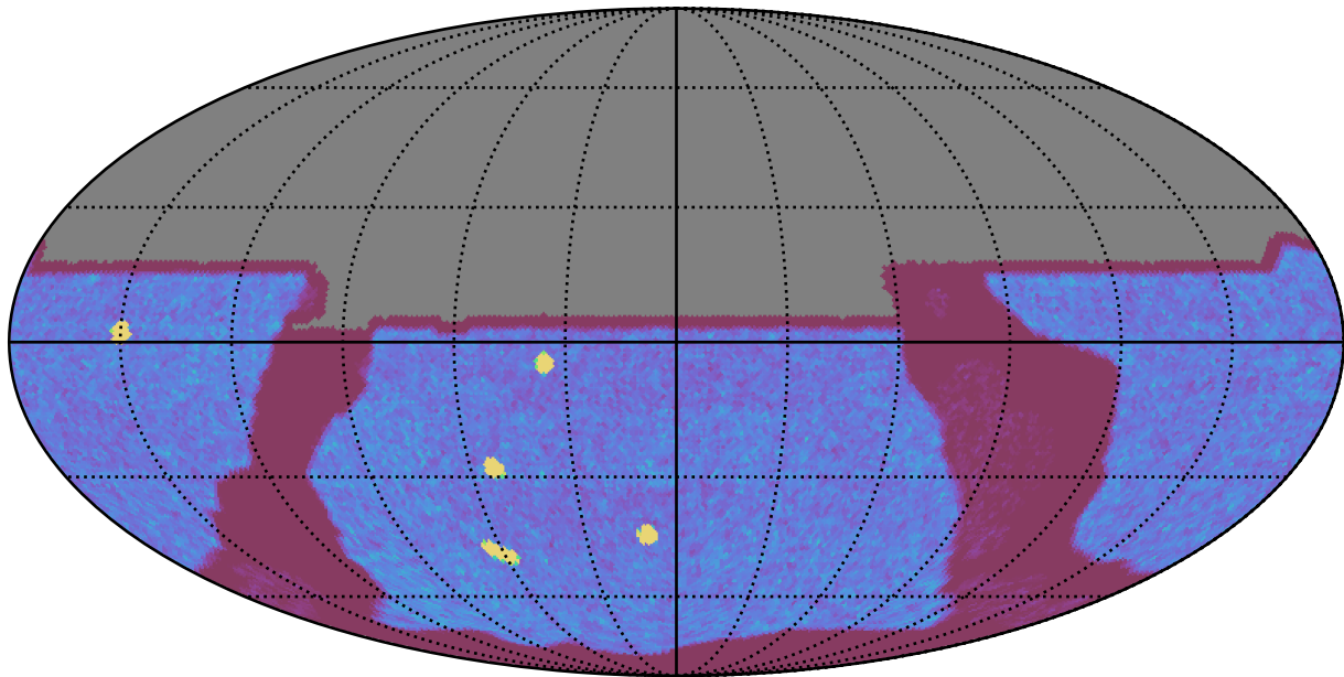
too_elab_r32_d3_griz_v3.4_10yrs All sky y band: NVisits
