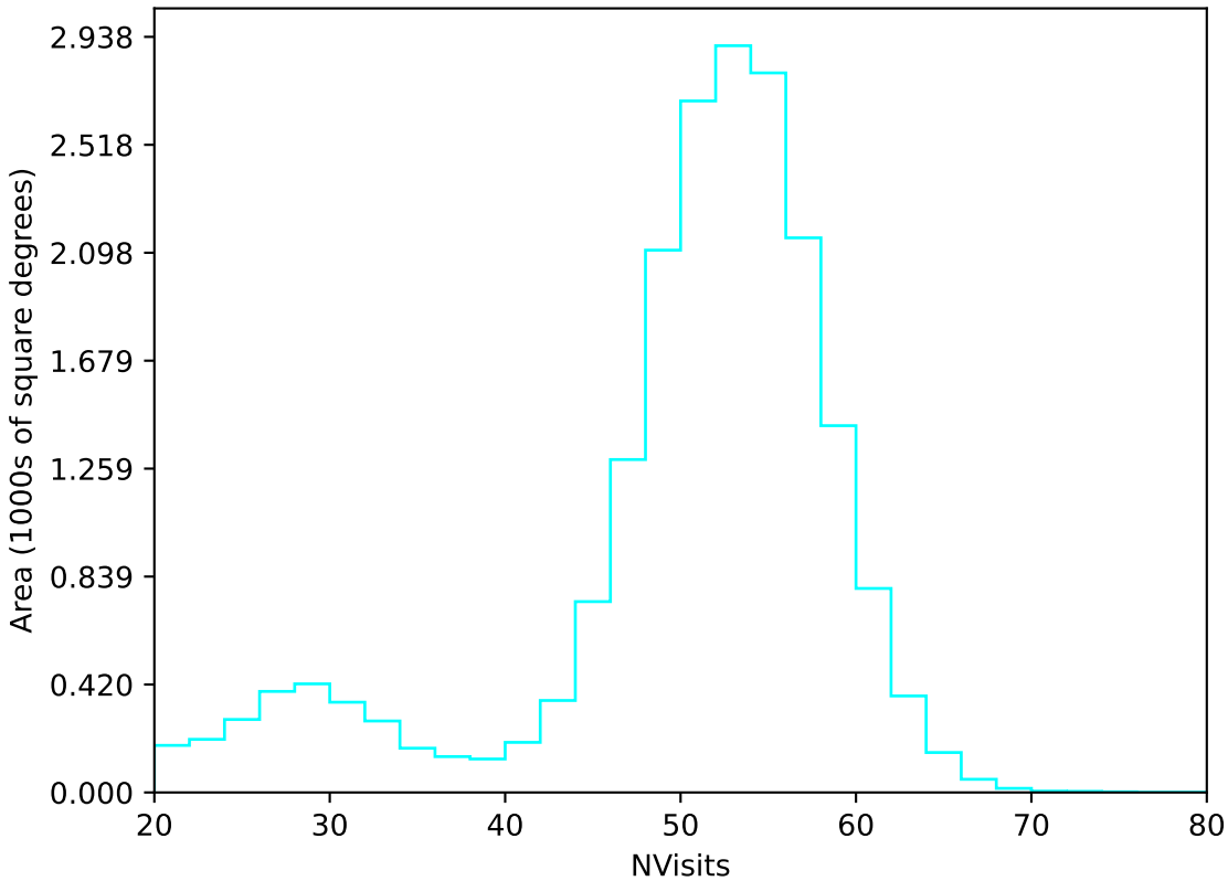
too_elab_r32_d3_griz_v3.4_10yrs All sky u band: NVisits
