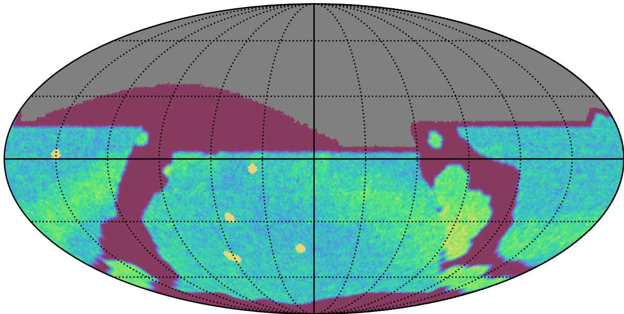
too_elab_r32_d3_griz_v3.4_10yrs All sky r band: NVisits
