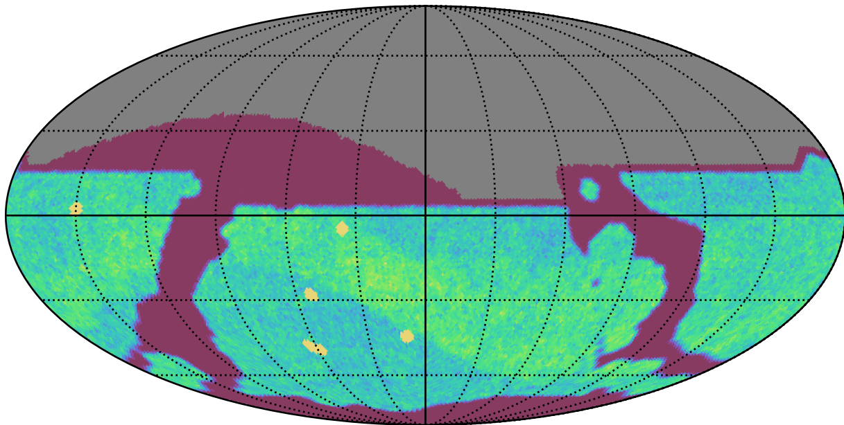
too_elab_r32_d3_griz_v3.4_10yrs All sky i band: NVisits
