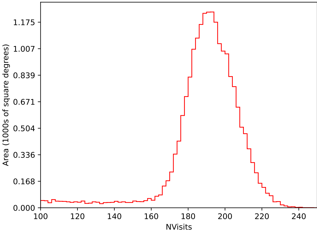
too_elab_r32_d3_griz_v3.4_10yrs All sky i band: NVisits
