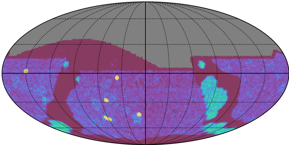
too_elab_r32_d3_griz_v3.4_10yrs All sky g band: NVisits
