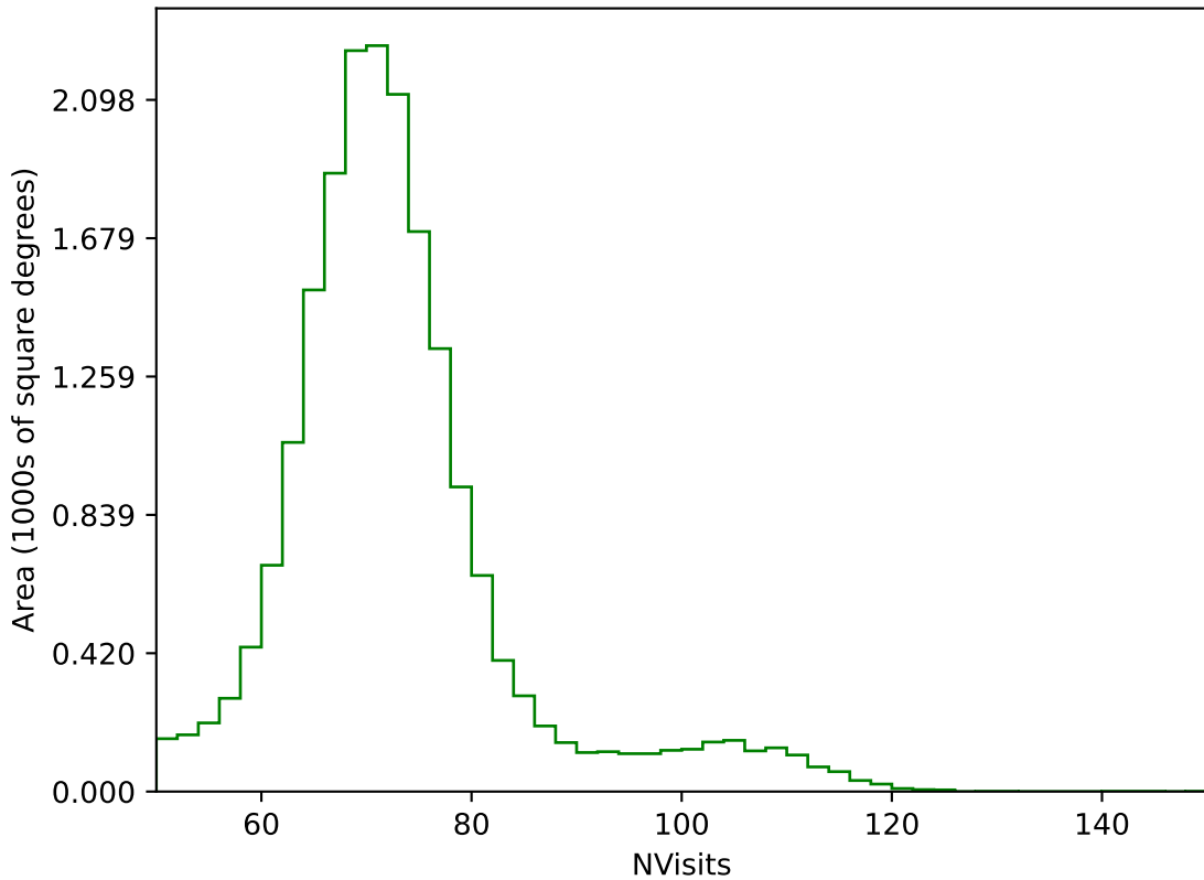
too_elab_r32_d3_griz_v3.4_10yrs All sky g band: NVisits
