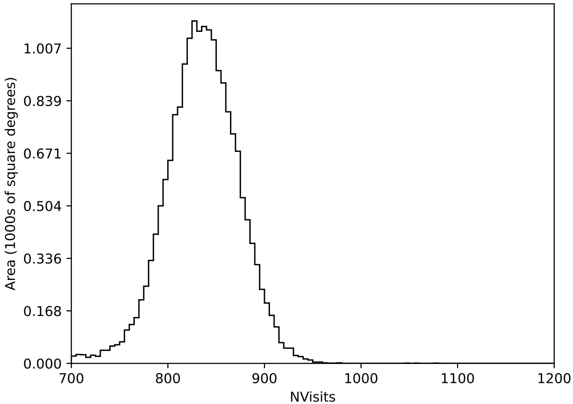
too_elab_r32_d3_griz_v3.4_10yrs All sky all bands: NVisits
