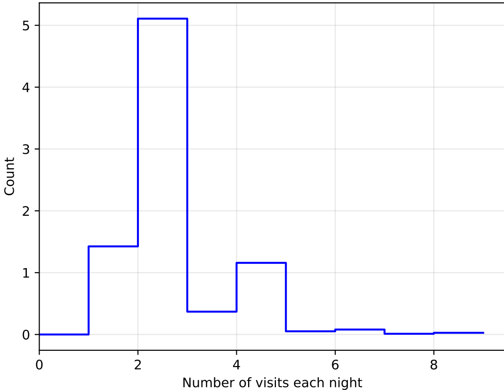
too_elab_r32_d3_griz_v3.4_10yrs WFD: NVisitsPerNight
