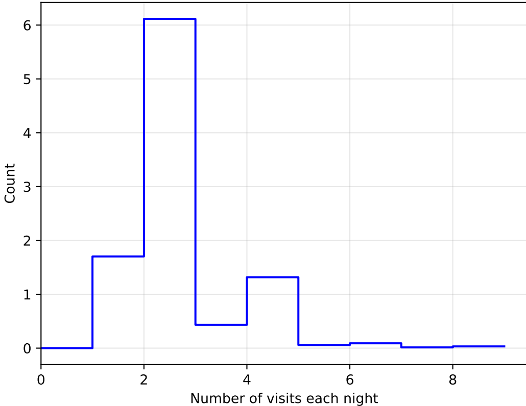
too_elab_r32_d3_griz_v3.4_10yrs All sky: NVisitsPerNight
