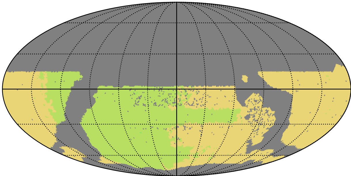
too_elab_r32_d3_griz_v3.4_10yrs WFD all bands: NSeasons
