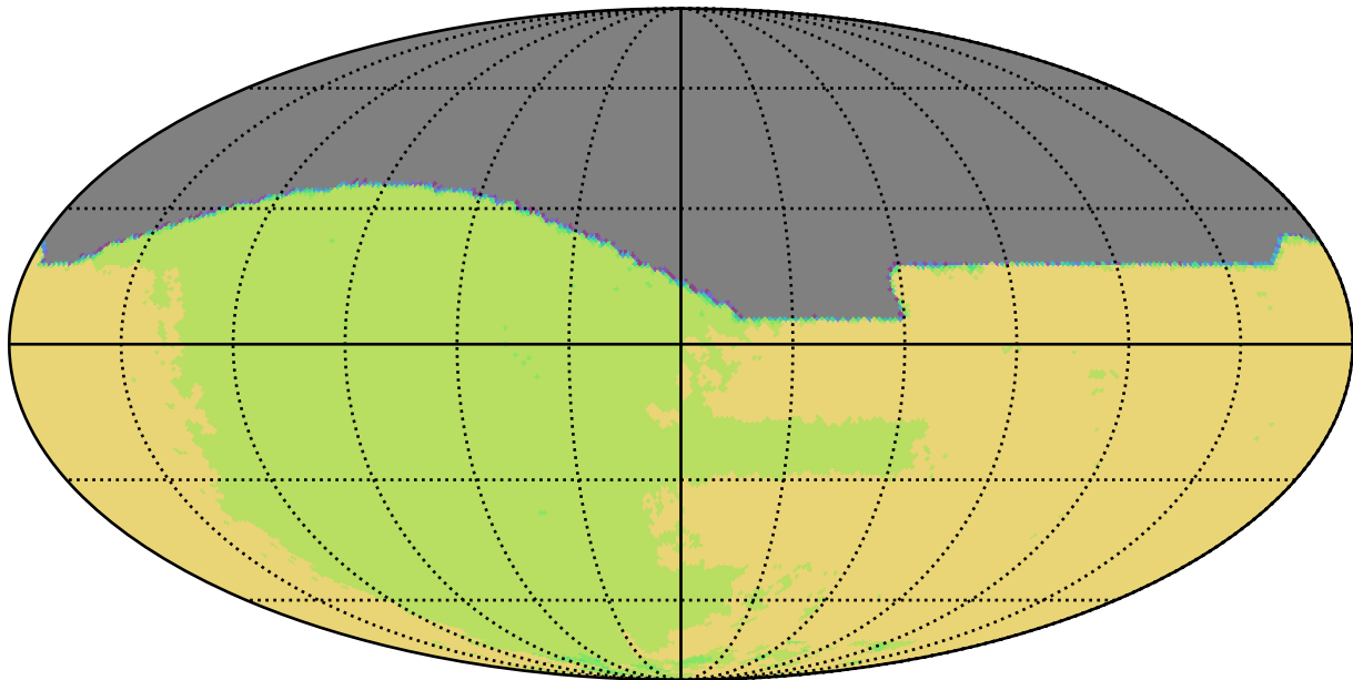
too_elab_r32_d3_griz_v3.4_10yrs All sky all bands: NSeasons
