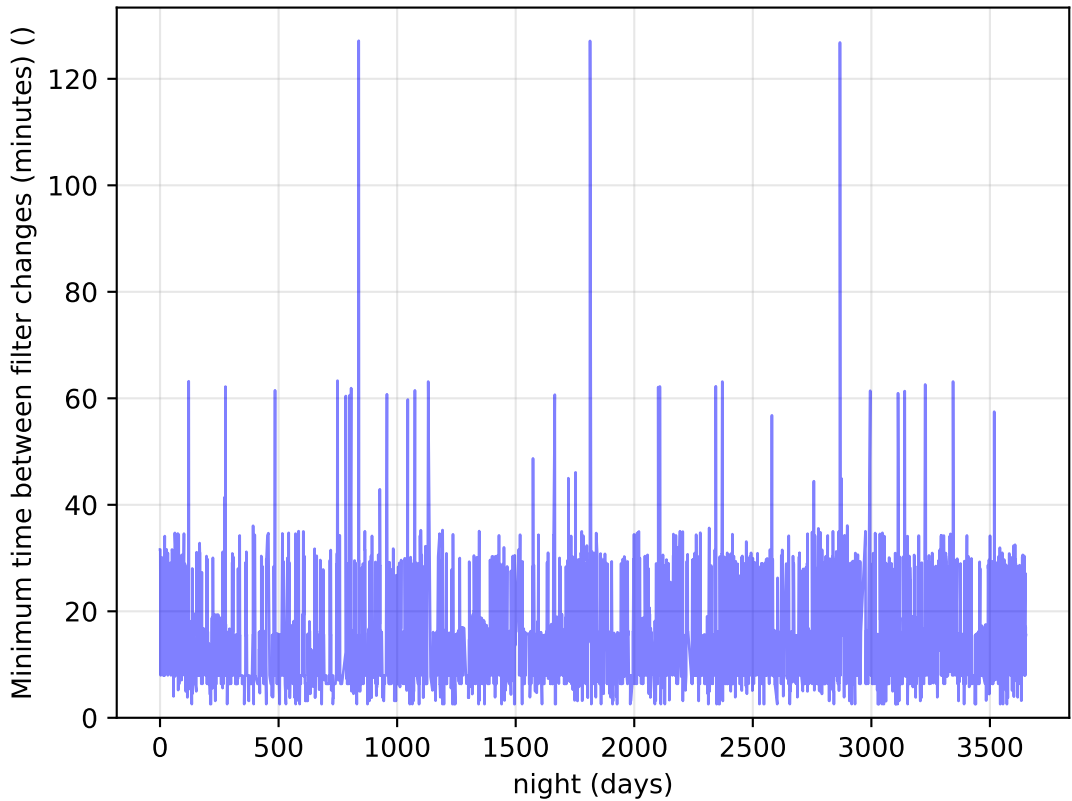
too_elab_r32_d3_griz_v3.4_10yrs Per Night: Minimum time between filter changes (minutes)
