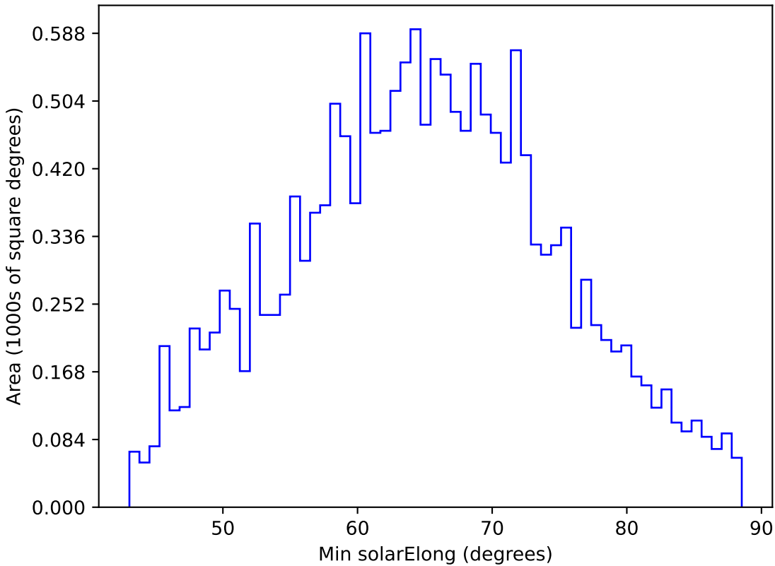
too_elab_r32_d3_griz_v3.4_10yrs WFD y band: Min solarElong
