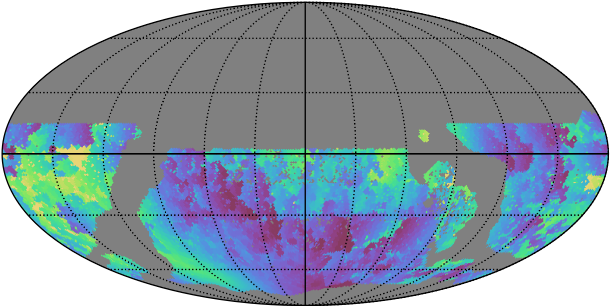
too_elab_r32_d3_griz_v3.4_10yrs WFD u band: Min solarElong
