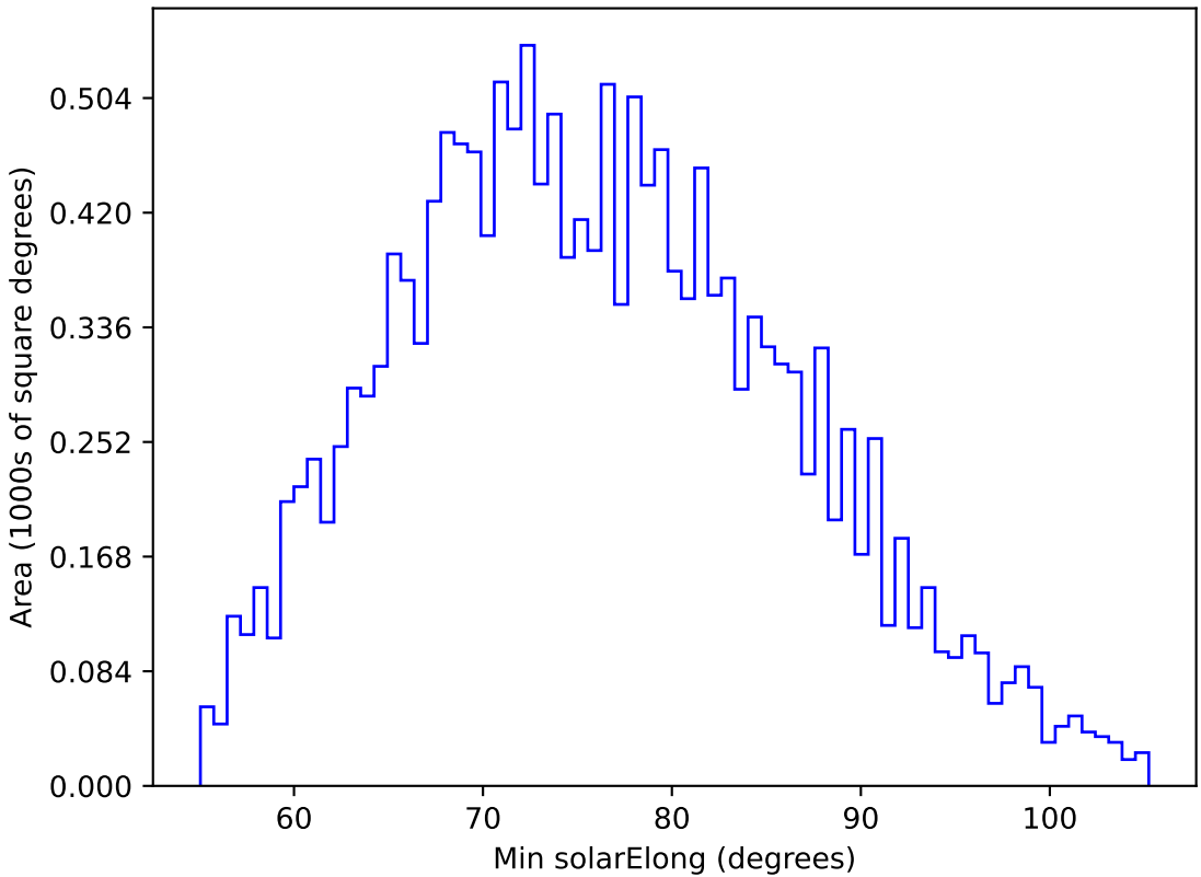
too_elab_r32_d3_griz_v3.4_10yrs WFD u band: Min solarElong
