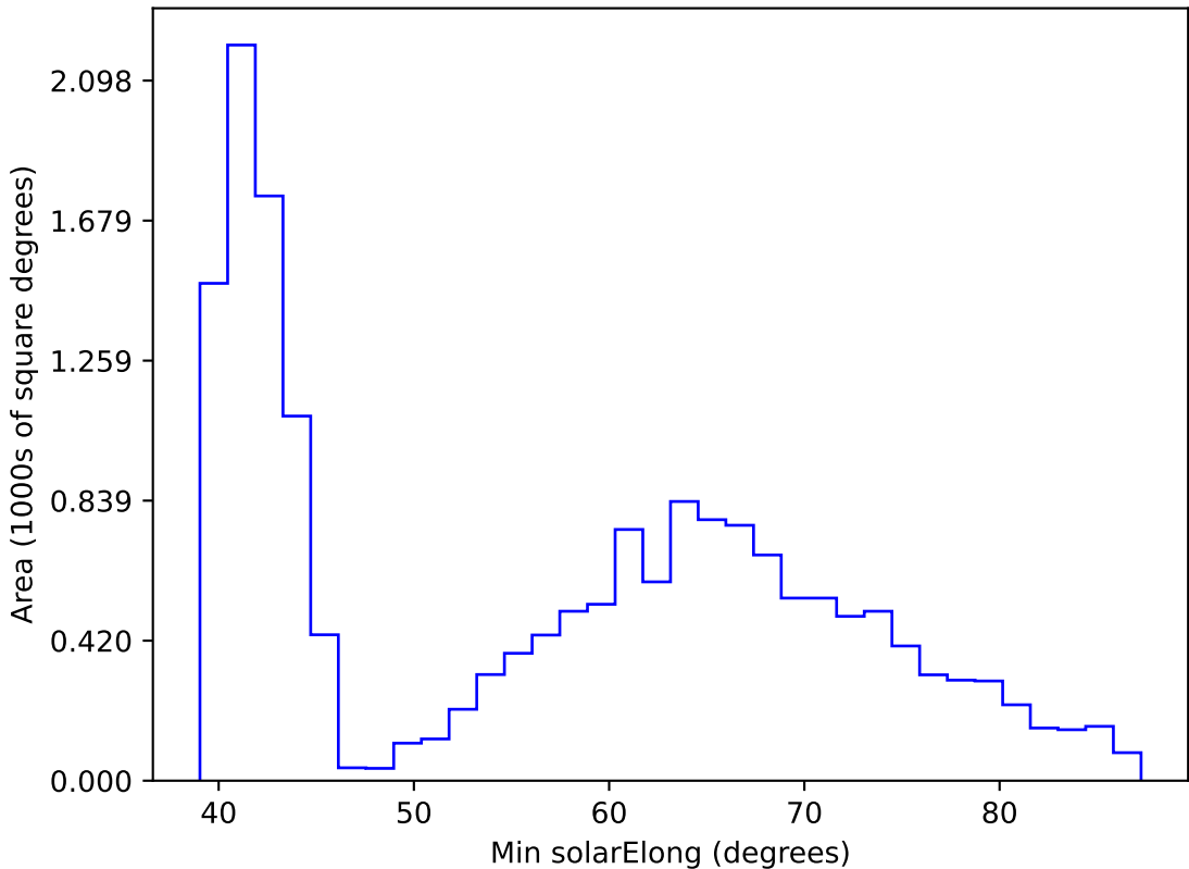
too_elab_r32_d3_griz_v3.4_10yrs WFD r band: Min solarElong
