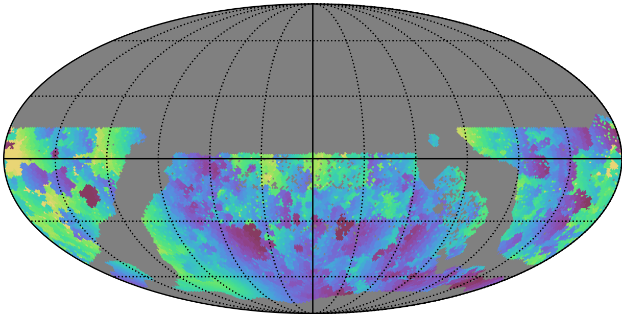
too_elab_r32_d3_griz_v3.4_10yrs WFD g band: Min solarElong
