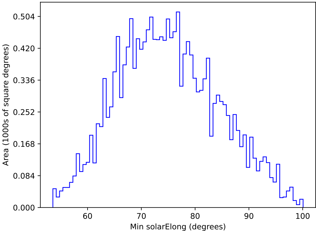
too_elab_r32_d3_griz_v3.4_10yrs WFD g band: Min solarElong
