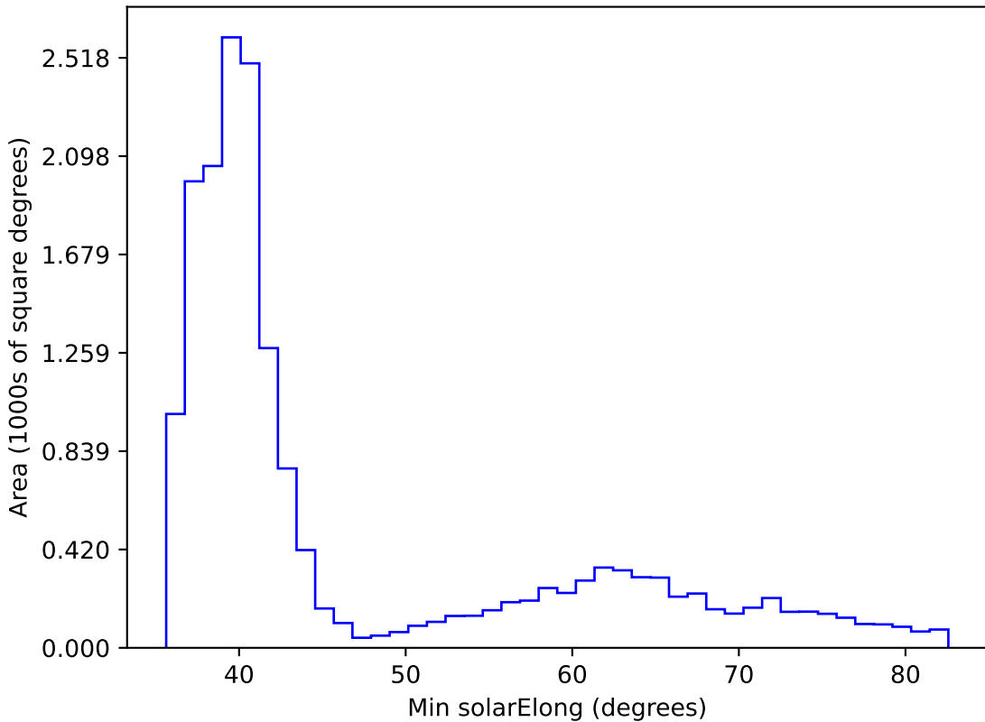
too_elab_r32_d3_griz_v3.4_10yrs WFD all bands: Min solarElong
